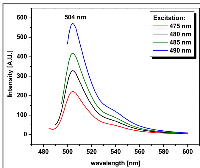
C11 TopFluor Galactosyl Ceramide Avanti Number 810266
